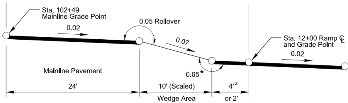
Figure 9-3 Maximum Grade Control Points in Gore Area
