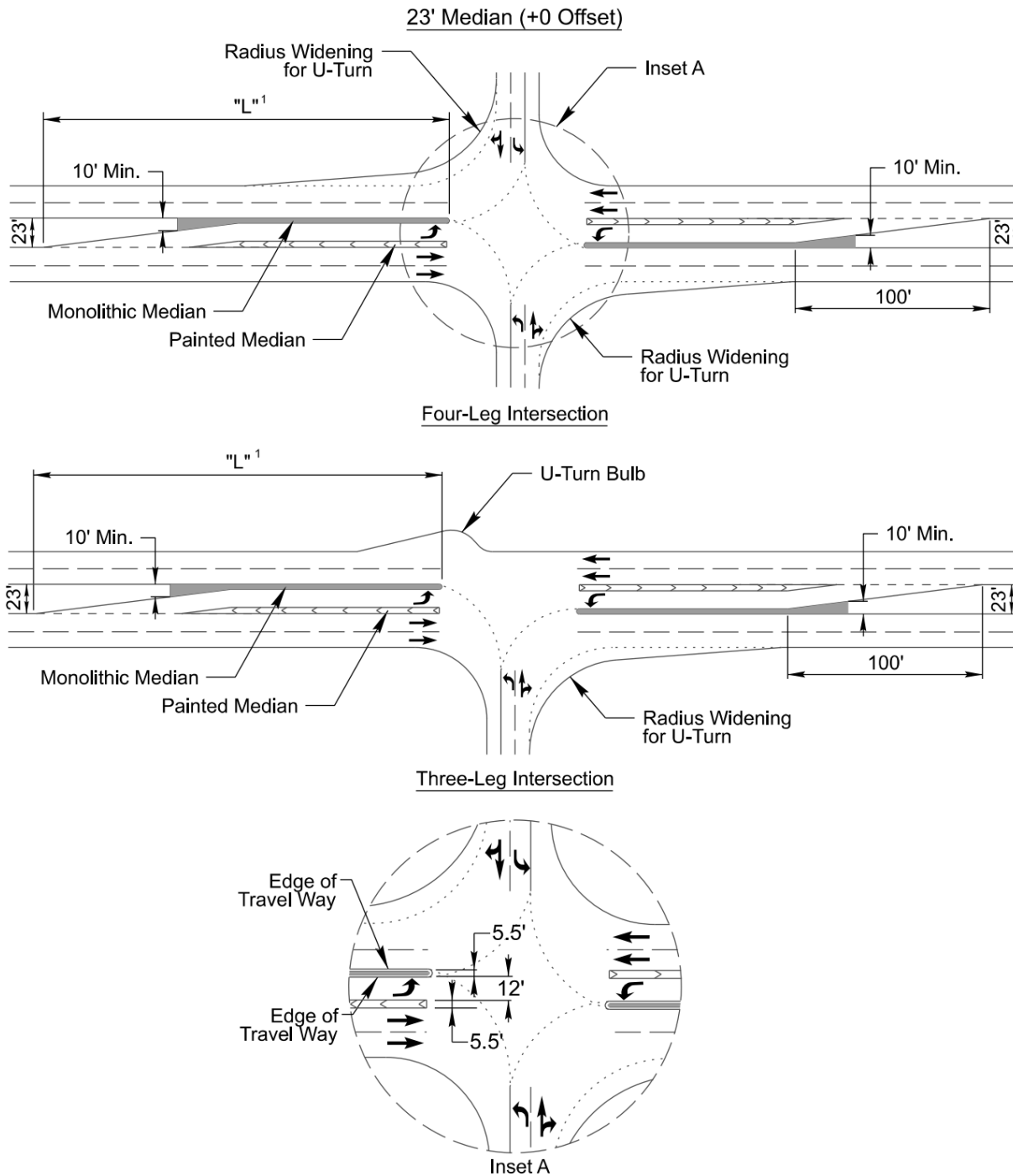
Figure 8-12 Guidelines for Offsetting Opposing Left Turn Lanes on Divided Roadways with a 23'0" Median
